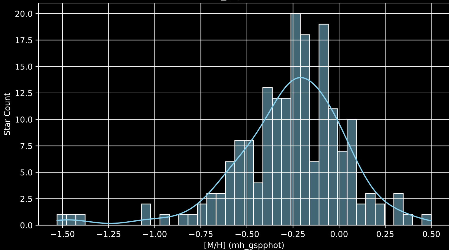
APOGEE DR17 Field: [CVZ_FILL03_btx [M/H] (mh_gspphot) (n= 182)
