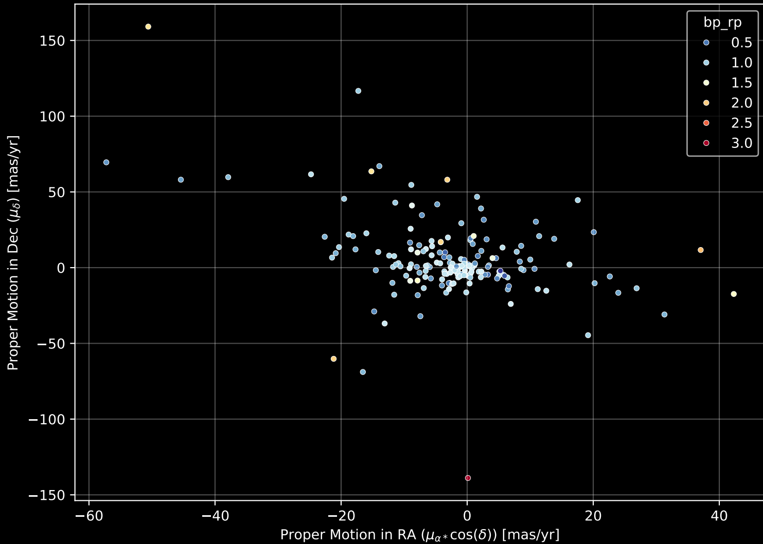
APOGEE DR17 Field: [CVZ_FILL03_btx] Proper Motion Diagram (n= 183)
