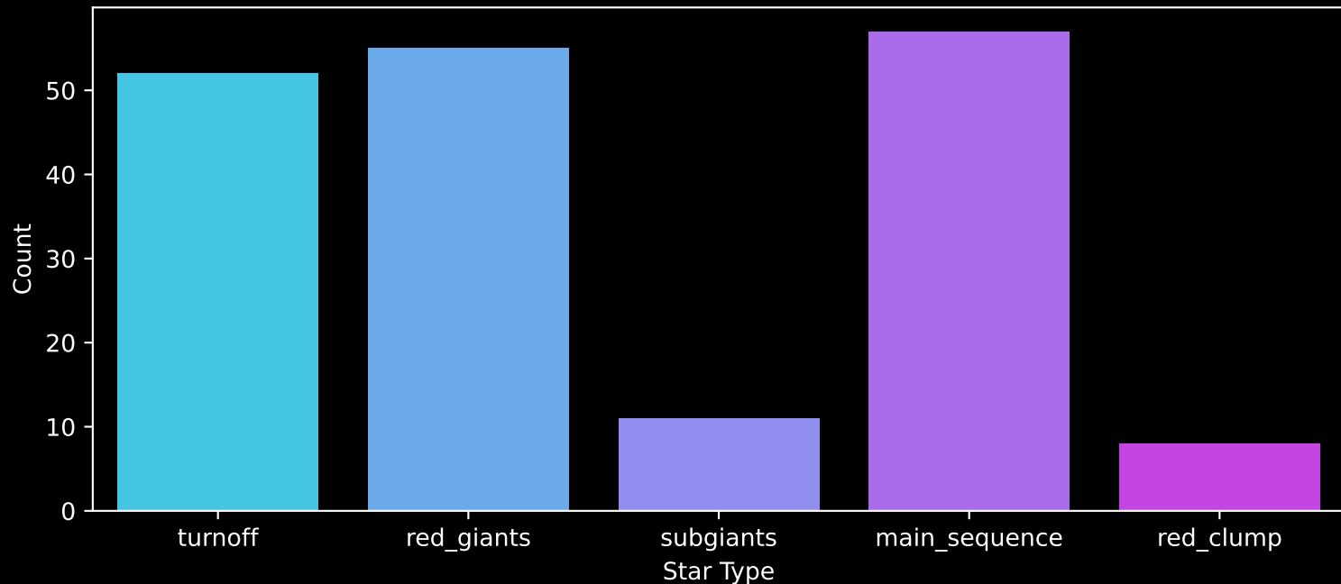
APOGEE DR17 Field: [CVZ_FILL03_btx] Count plot of Star Type
