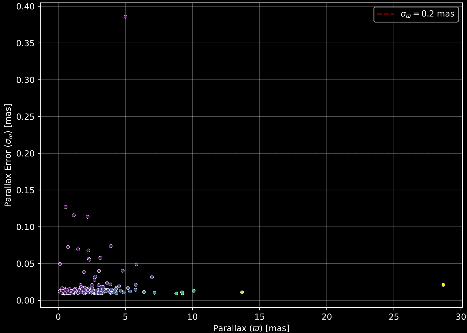
APOGEE DR17 Field: [CVZ_FILL03_btx] Parallax Quality (n= 183)
