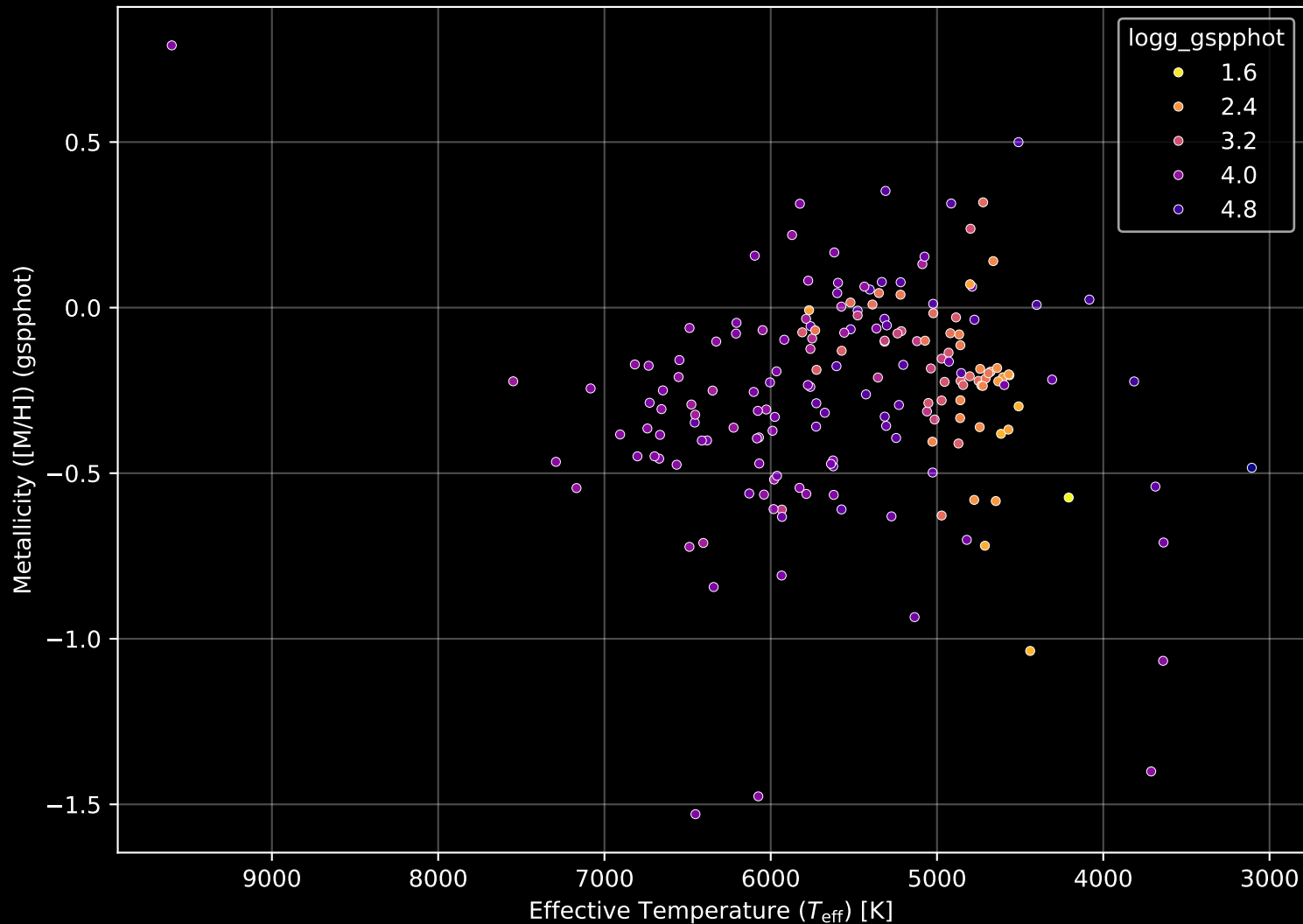
APOGEE DR17 Field: [CVZ_FILL03_btx] Stellar Population Parameters (n= 183)
