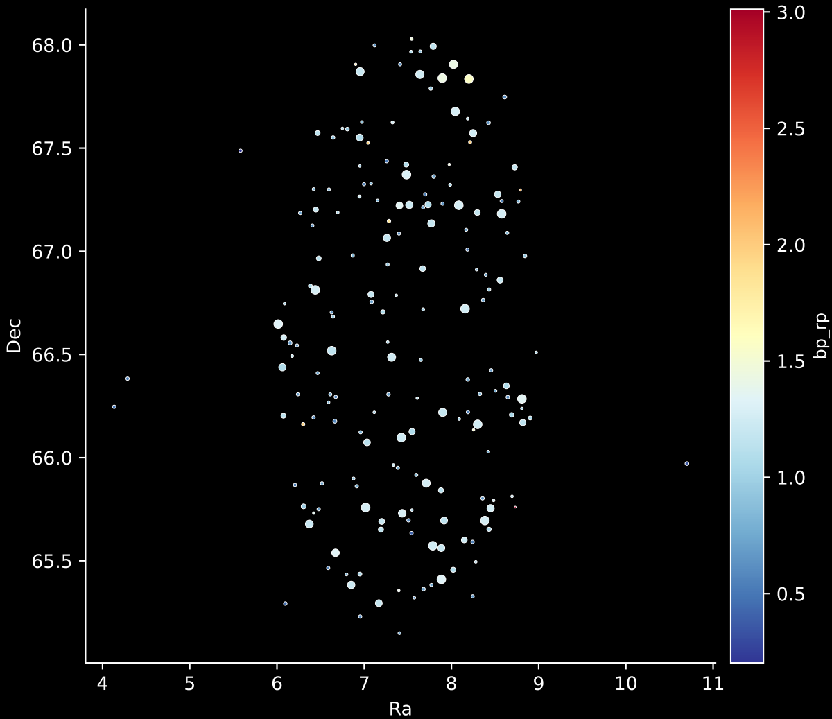
APOGEE DR17 Field: [CVZ_FILL03_btx] Stars: 183
