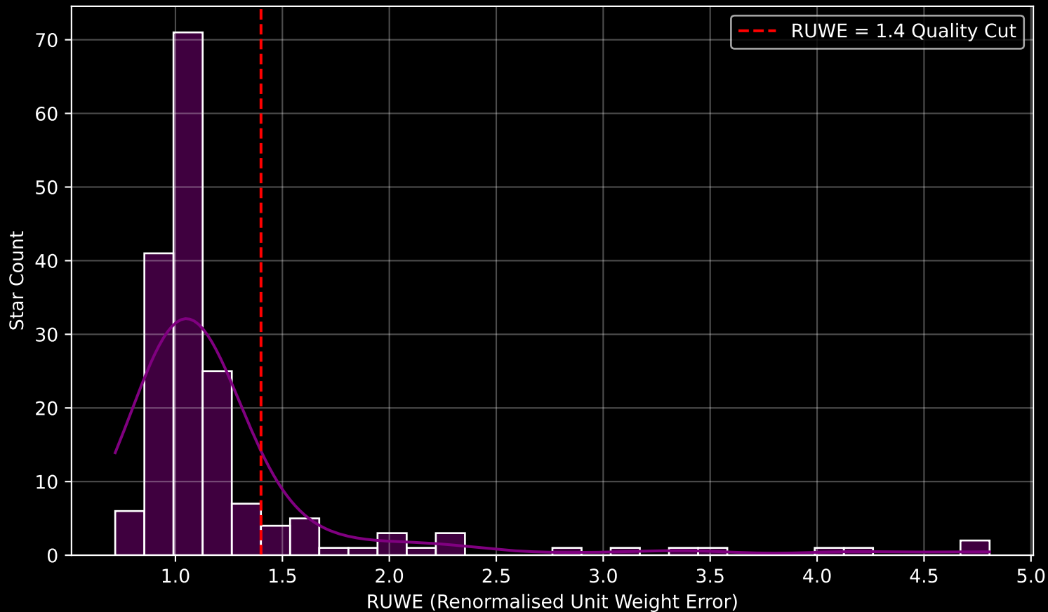
GAPOGEE DR17 Field [CVZ_FILL03_btx] RUWE Distribution (n= 176)
