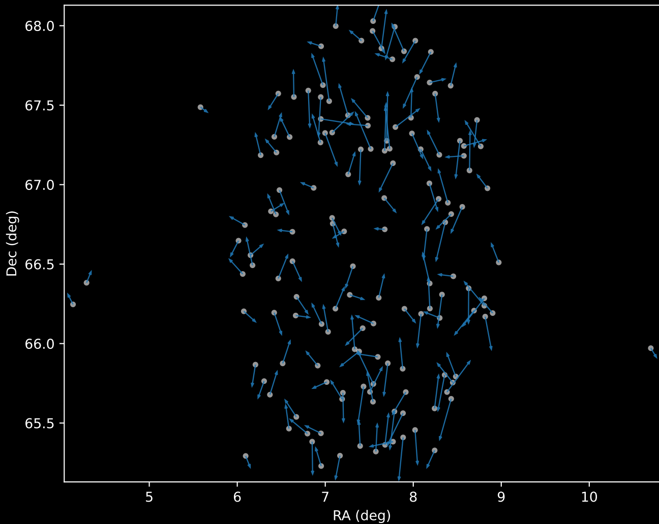
APOGEE DR17 Cluster 0 Proper Motion Vectors (n=146)
